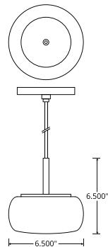
STANDARD CANOPY
