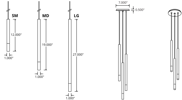
CYLINDER SIZES
